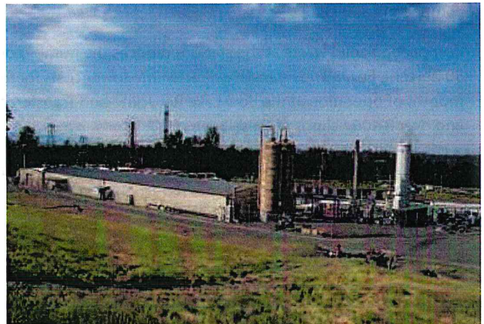
The Bio Energy Washington plant at Cedar Hills landfill converts landfill gas to pipeline quality gas
