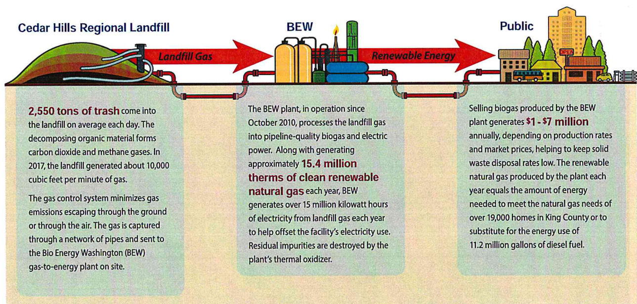
Figure 2-6. Landfill gas-to-energy process
